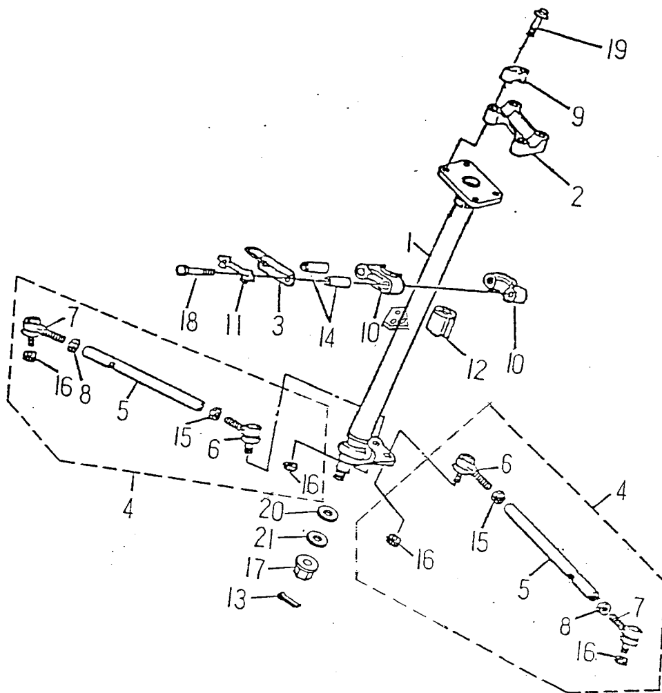
FIG.18 STEERING 轉向裝置
