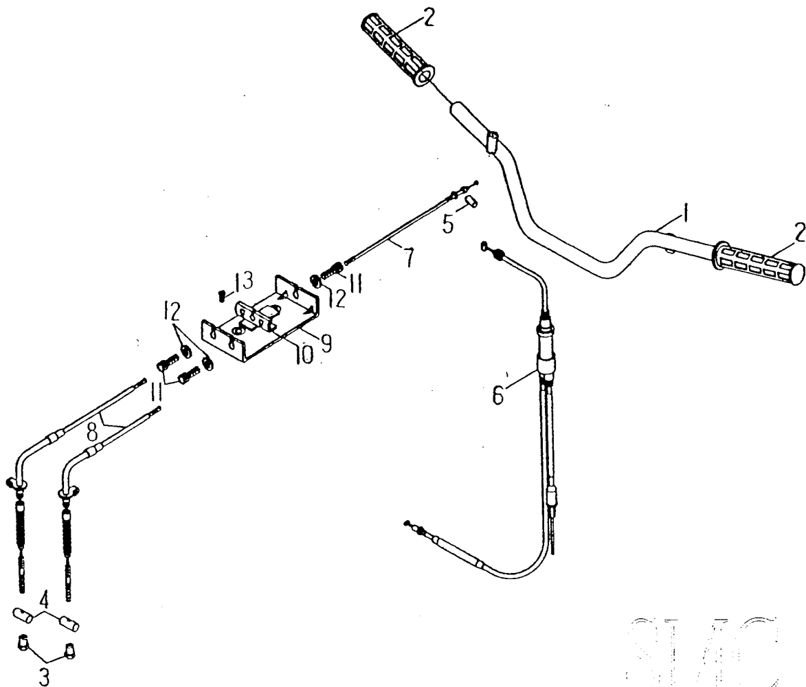
FIG.25 STEERING HANDLE CABLE 轉向把手,鋼索
