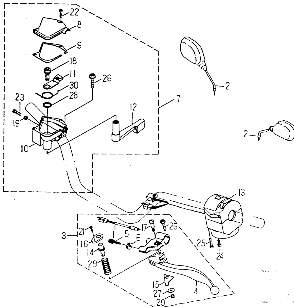
FIG.26 HANDLE SWITCH , LEVER 把手開關,拉桿
