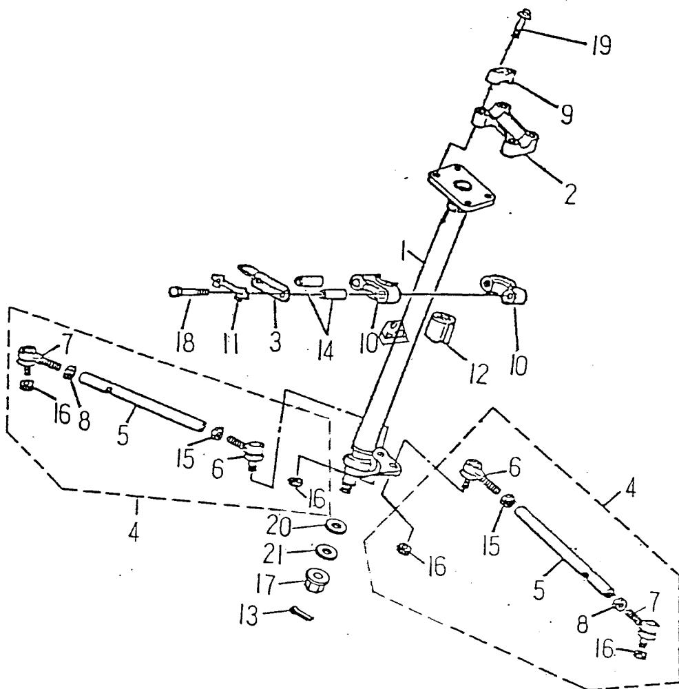
FIG.18 STEERING 轉向裝置
