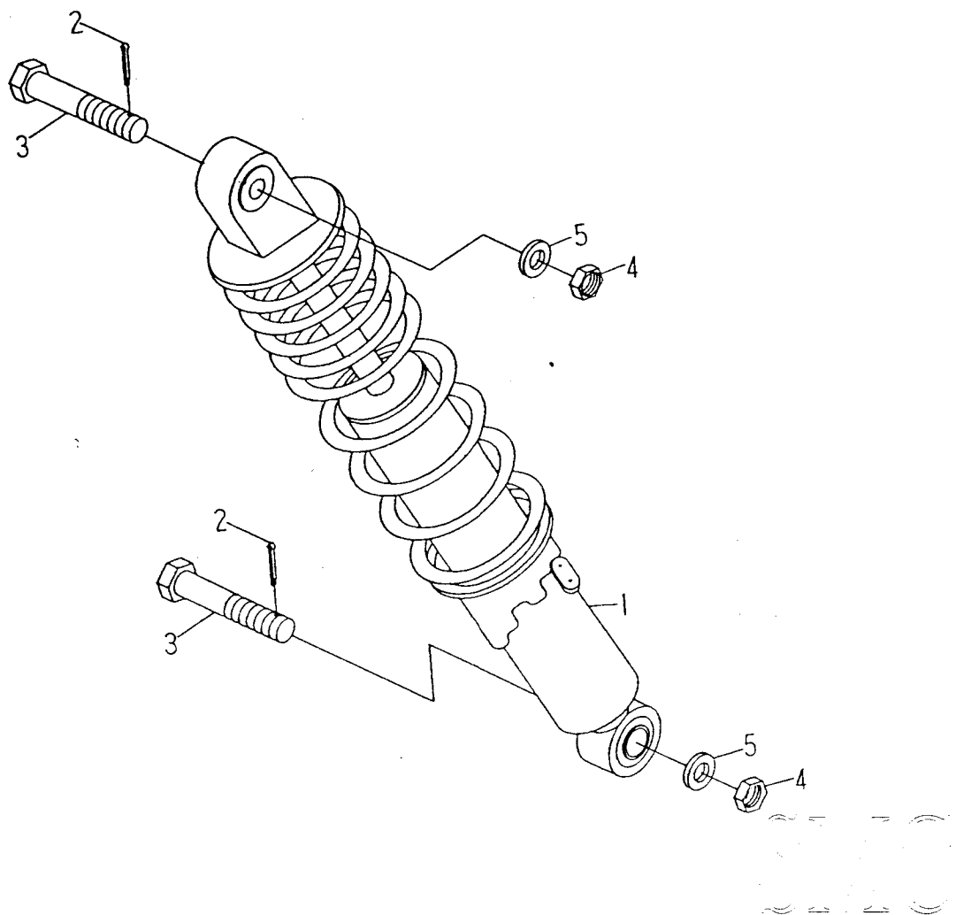
FIG.15 REAR SUSPENSION 後懸吊系統
